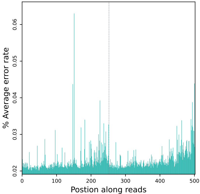
Error rate distribution along reads (R10517)
